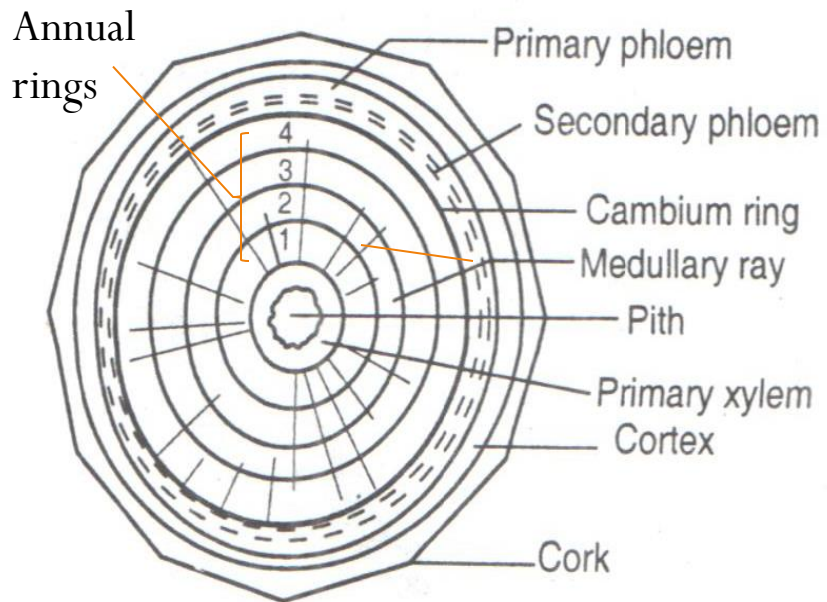
Fig. 4.13: Annual rings
